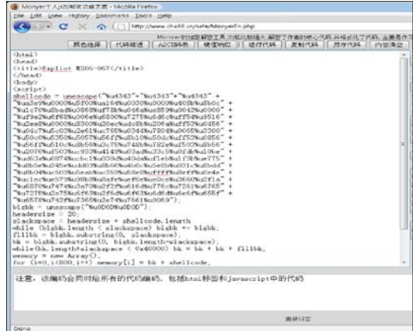
Figure 3: One of cha88's script / css / html encoder / decoder user interfaces
