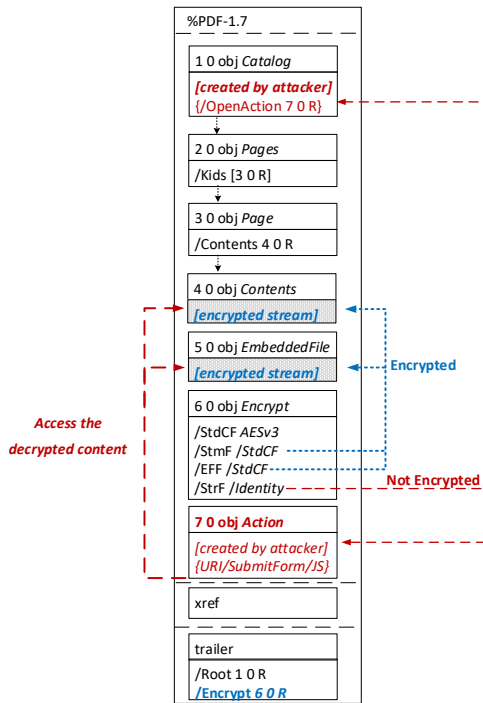
Figure 5: A PDF file modified by the attacker. Once the file is opened, the victim enters the correct password as usual, but due to the modification, the decrypted stream of objects 4 and 5 is automatically sent to an attacker-controlled server.
