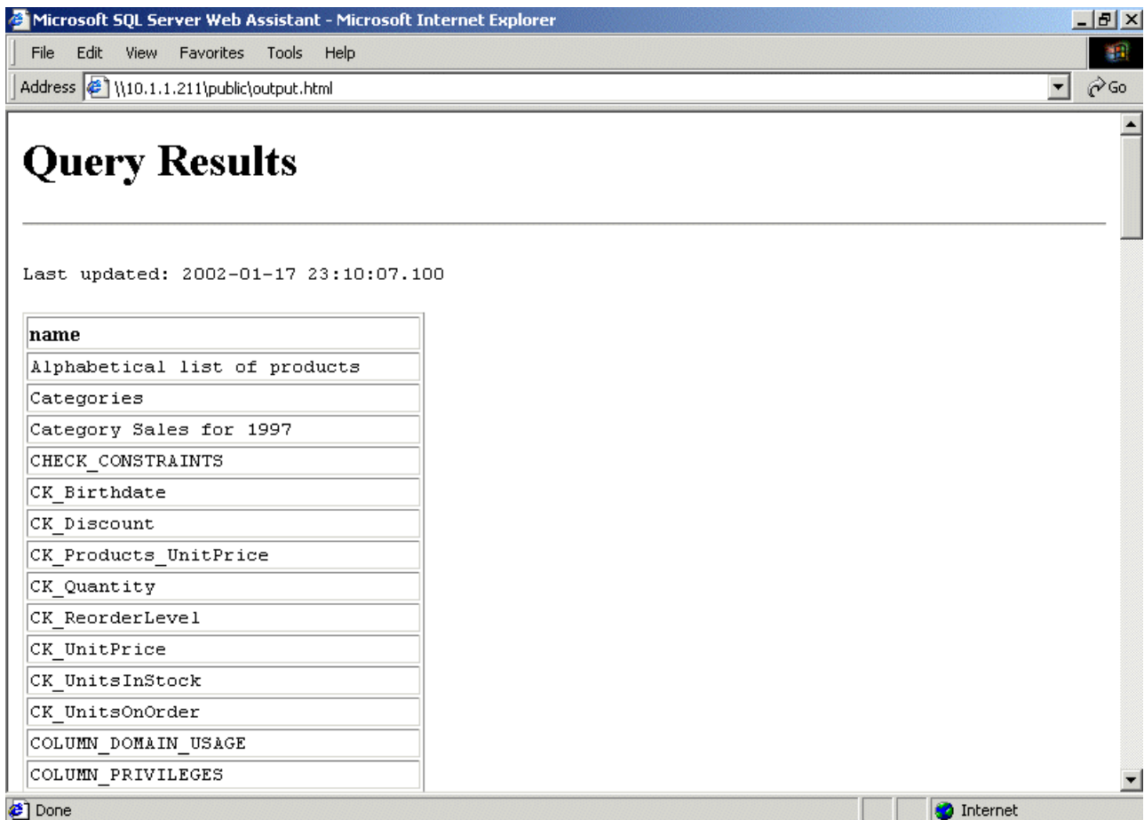
Figure 9: Using sp_makewebtask
